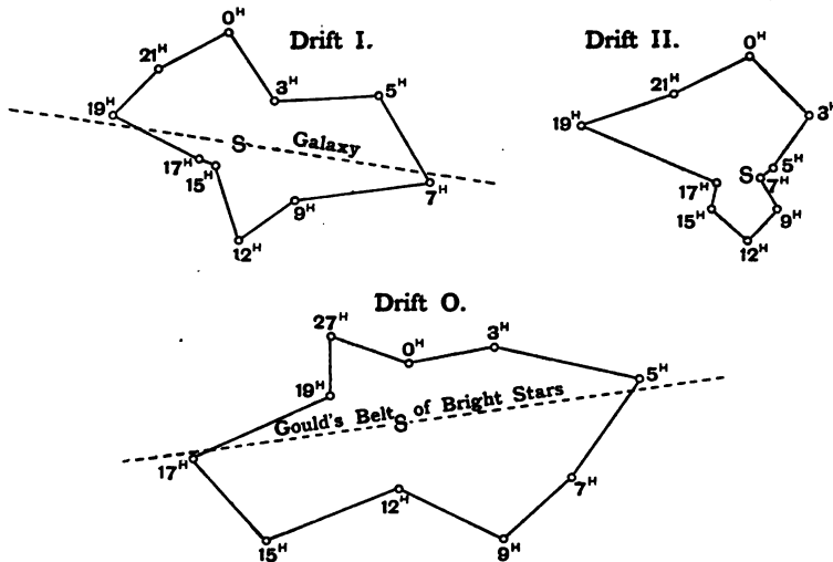
FIG. 17.—Distribution of Drifts along the Equator (Halm).
